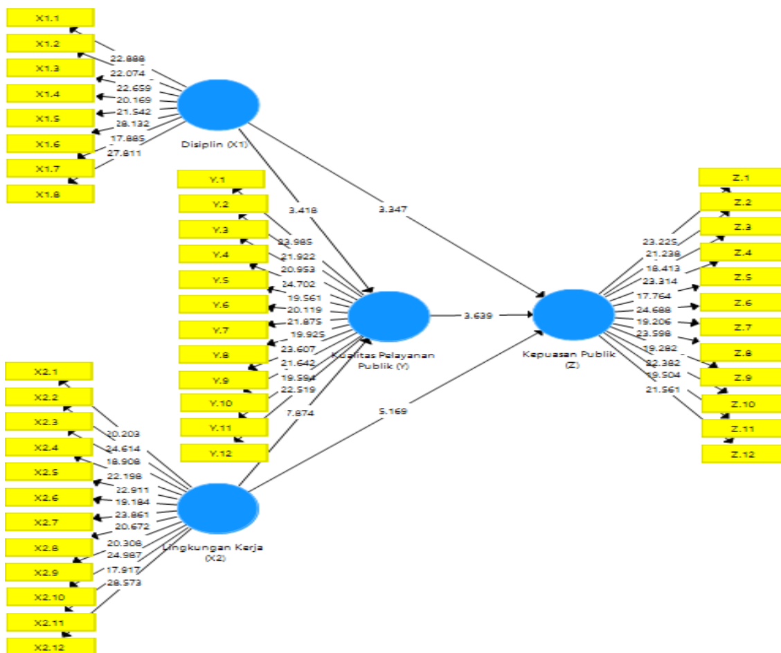
Figure 2. Bootstrapping
